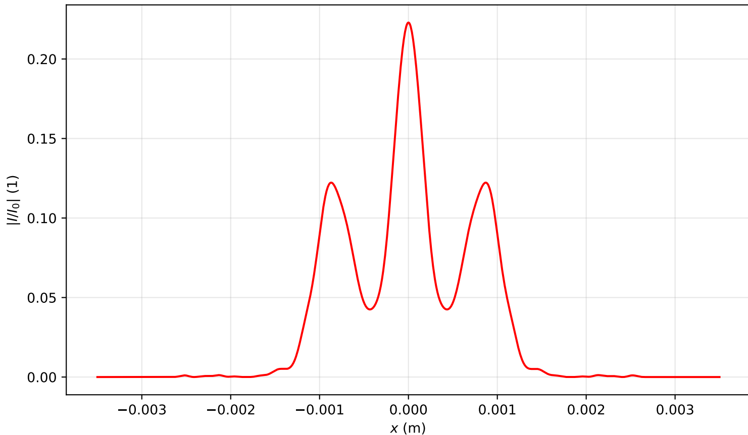
Intensity profile I(x, y = 0, z = 2.149)/I_0 , P_{in}=7.5P_{cr} , artificial time
